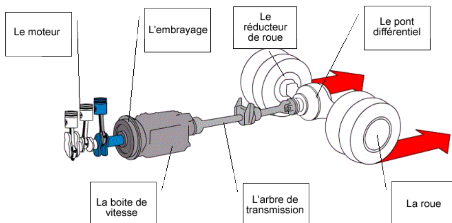
Figure 7: Circuit de transmission mécanique
