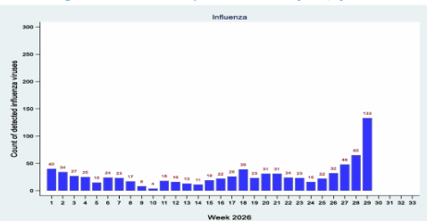
Figure 2. Influenza viruses reported since 1 January 2026, by week
